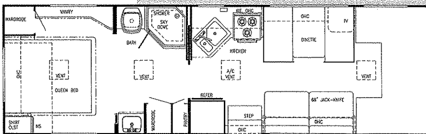
Model W6301D (Twin Beds or Bunks Opt.)
