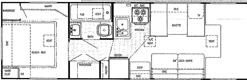
Model W6294D (Twin Beds or Bunks Opt.)
