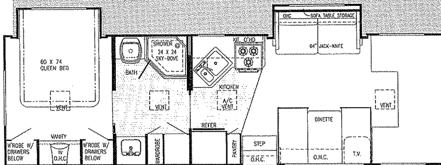
Model 6302D - (Twin Beds or Bunks Opt.)
