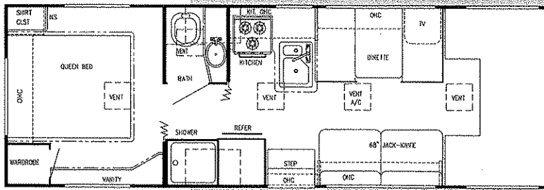
Model W6272D (Twin Beds or Bunks Opt.)
